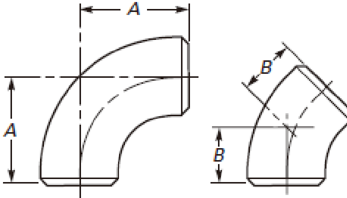
Dimensions of Elbows
