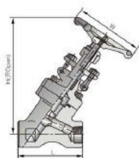
螺栓连接阀盖，缩径和全径，明杆支架 (OS & Y) Bolted bonnet, full port reducing port outside screw and yoke(OS & Y) 末端连接为螺纹或承插焊对接，设计按BS5352 Threaded, butt-welded or socket welded eds; design to BS5352
